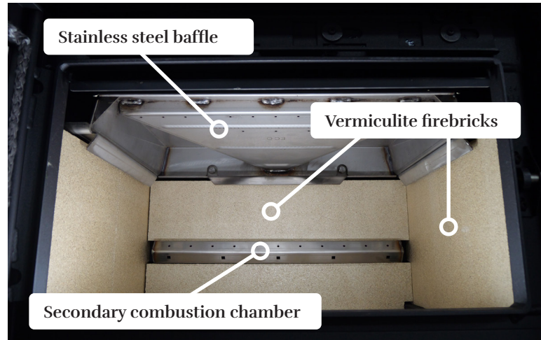
The firebox of the Monte ECO is designed to stay hotter for longer and reburn smoke particles.
