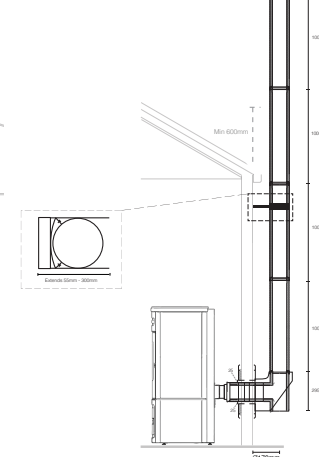
Room Sealed PELLET Flue Kit Rear Pellet Flue Kit
