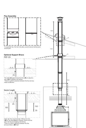
Insulated Room Sealed Flue Kit 5m Flue Kit for Cast Iron Fireplaces
