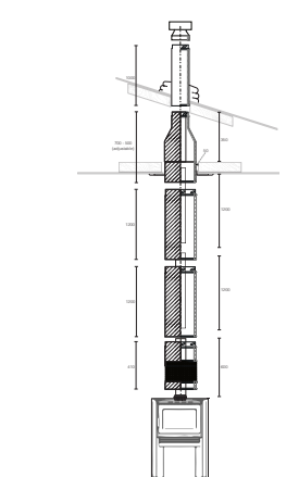
Insulated Room Sealed Flue Kit Standard Ceiling Enviro Flue Kit
