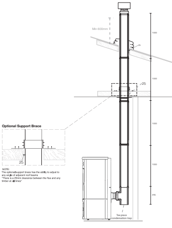
Room Sealed PELLET Flue Kit 4m Vertical Pellet Flue Kit
