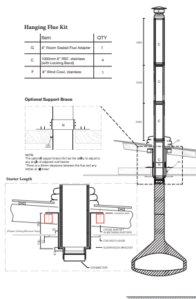
Insulated Room Sealed Flue Kit Flue Kit for Hanging Fireplaces
