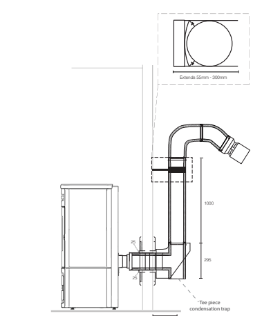
Room Sealed PELLET Flue Kit Rear Snorkel Pellet Flue Kit
