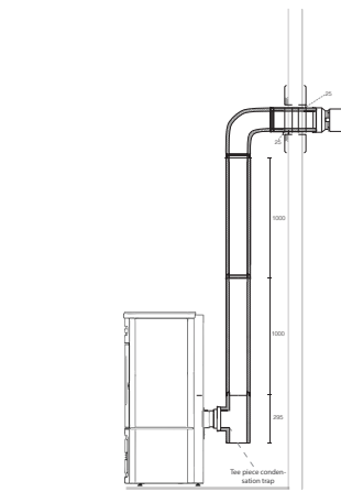
Room Sealed PELLET Flue Kit 4m Vertical Snorkel Pellet Flue Kit
