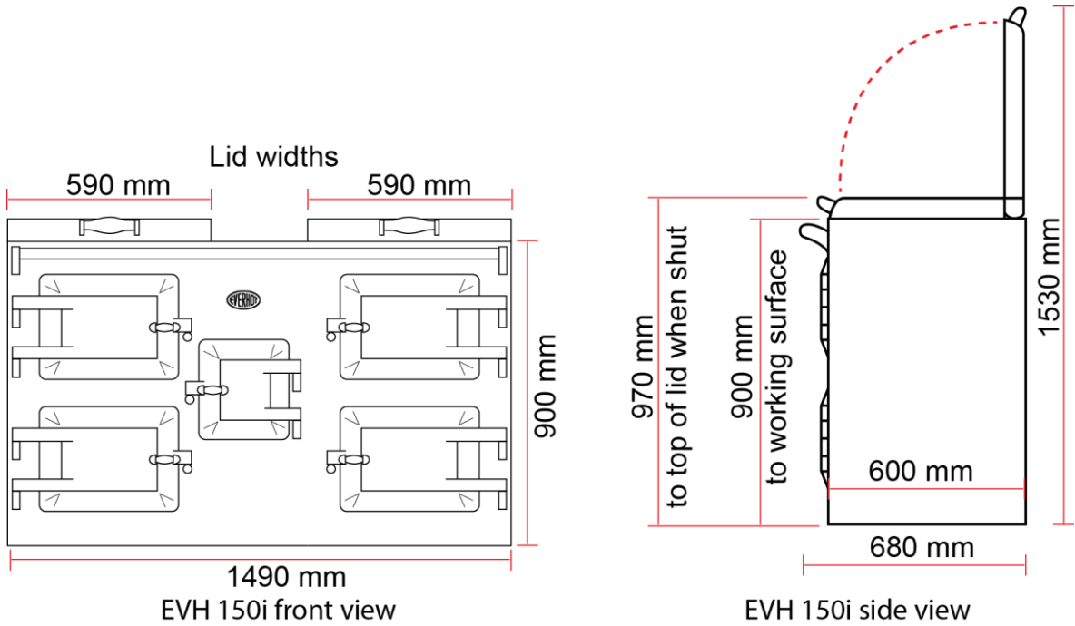
EVH150i dimensions
